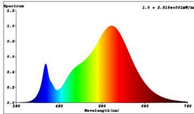
Spectral power distribution for FH-VL-U-10VWV
